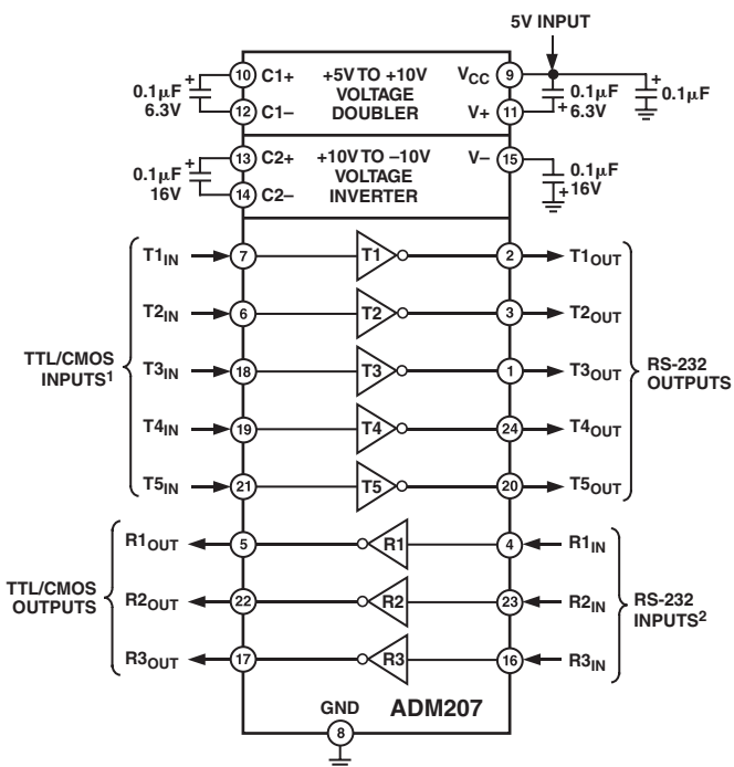
Figure 4. ADM207 Typical Operating Circuit
