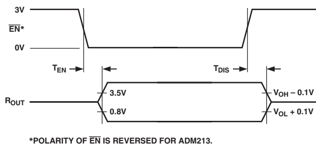
Figure 15. Enable Timing
