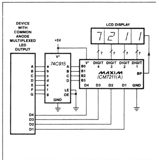
Figure 21. Multiplexed LED Driver to LCD Interface.
