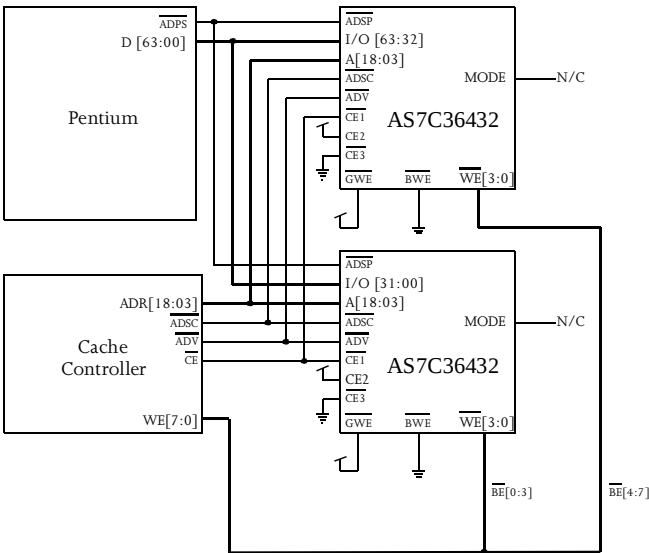
Figure A: Pentium 512KB single bank cache
