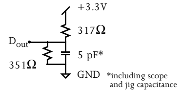
Figure C: Output load(B) for t_{LZC} , t_{LZOE} , t_{HZOE} , t_{HZC}
