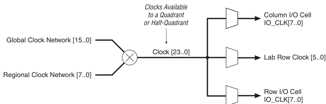
Figure 1–41. Hierarchical Clock Networks Per Quadrant
