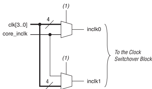
Figure 1–43. Enhanced PLL Clock Input Multiplex Logic
