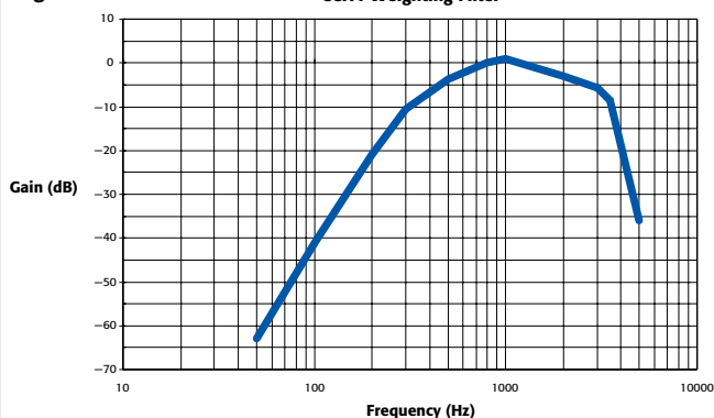
CCITT Weighting Filter
