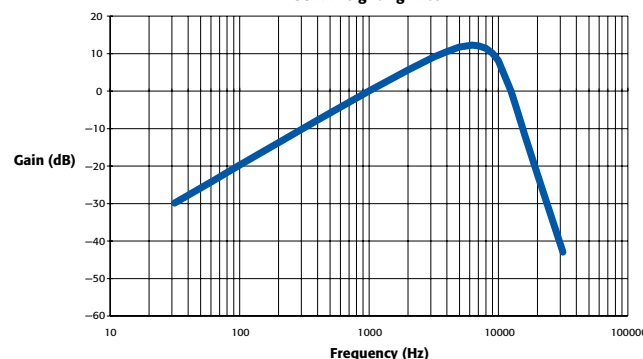
CCIR Weighting Filter
