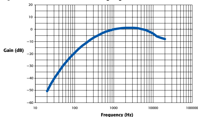
A Weighting Filter
