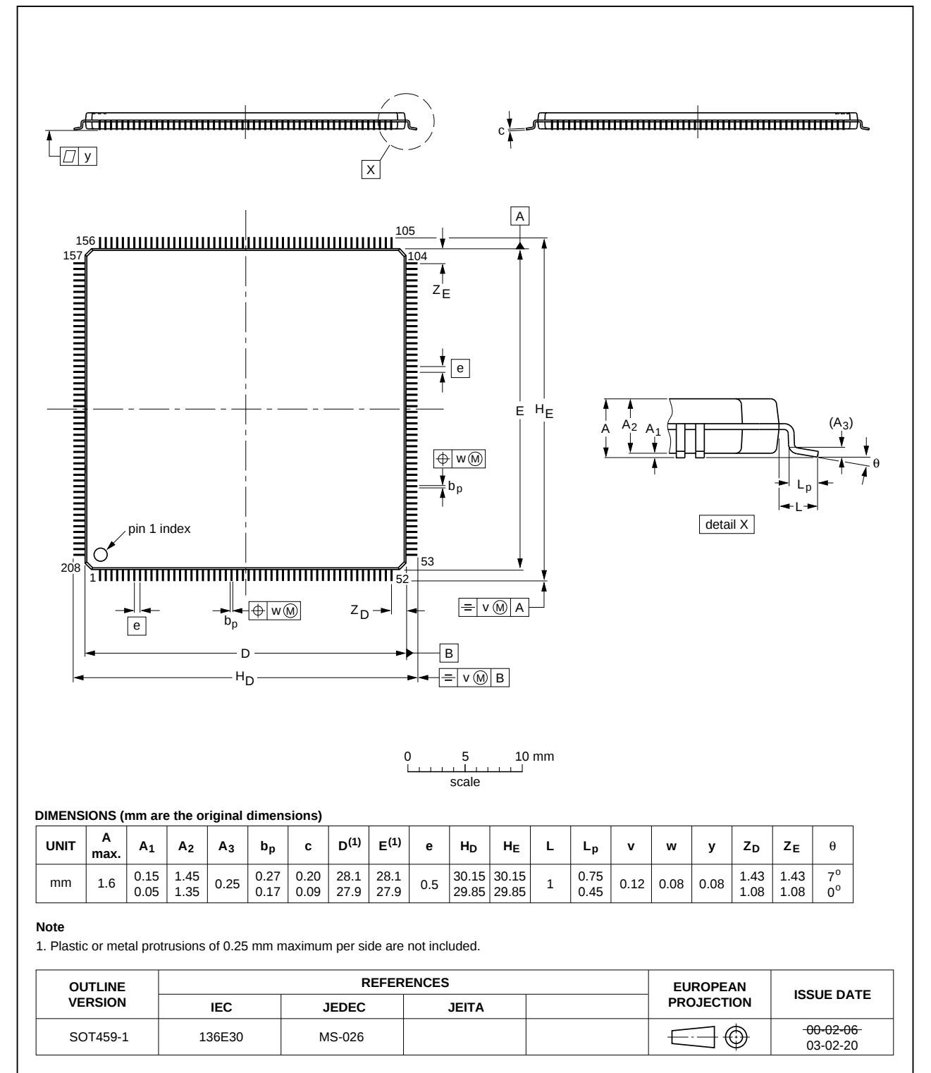
Fig 50. Package outline of the LQFP208 package
