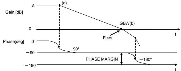
Figure 52. Bode Plot
