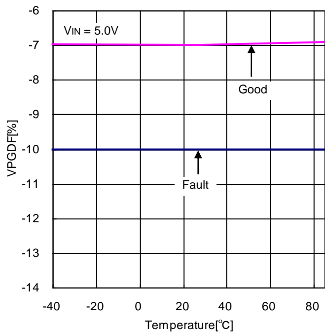
Figure 16. PGD Falling Voltage vs Temperature
