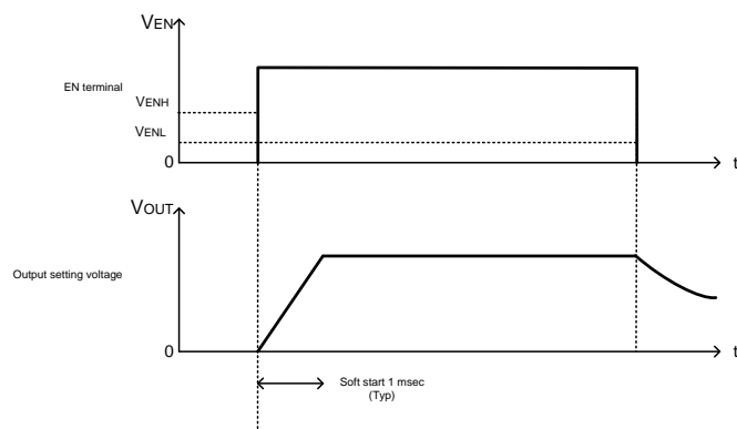
Figure 43. Start Up and Down with Enable
