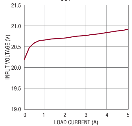
Minimum Required Input Voltage vs Load 18V_{OUT}
