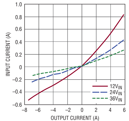
Input Current vs Output Current 1.2V OUT
