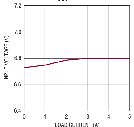
Minimum Required Input Voltage vs Load 5V_{OUT}
