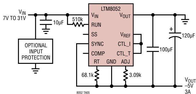
31V IN , -5V OUT Negative Converter
