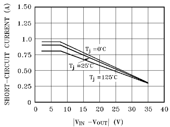
SHORT-CIRCUIT CURRENT
