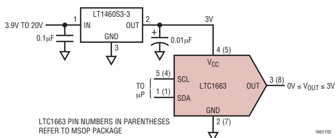
Figure 2. LT1460 As Power Supply for the LTC1663
