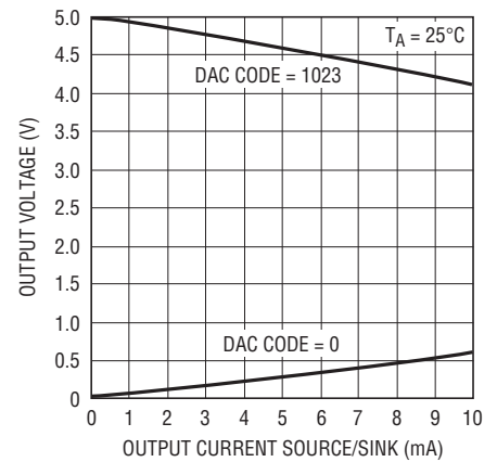
Source and Sink Current Capability with V_{CC} = 5\text{V}
