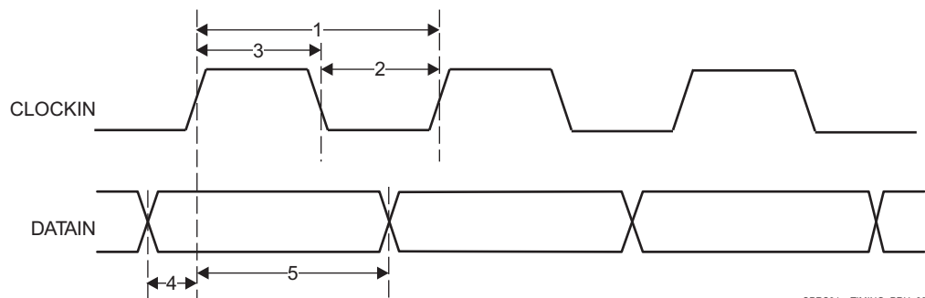
Figure 5-106. PRU-ICSS PRU Parallel Capture Timing - Rising Edge Mode
