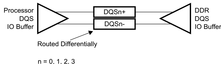
Figure 7-22. DQS Topology
