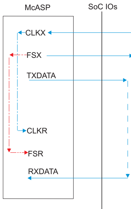
Figure 5-61. McASP1-8 CI-FO- – SYNC Mode
