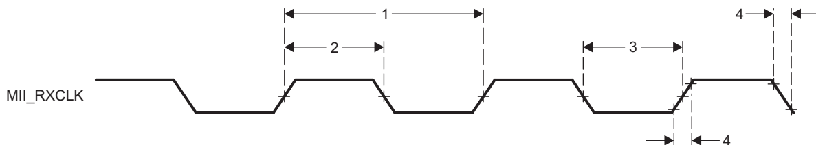
Figure 5-120. PRU-ICSS MII[x]_RXCLK Timing
