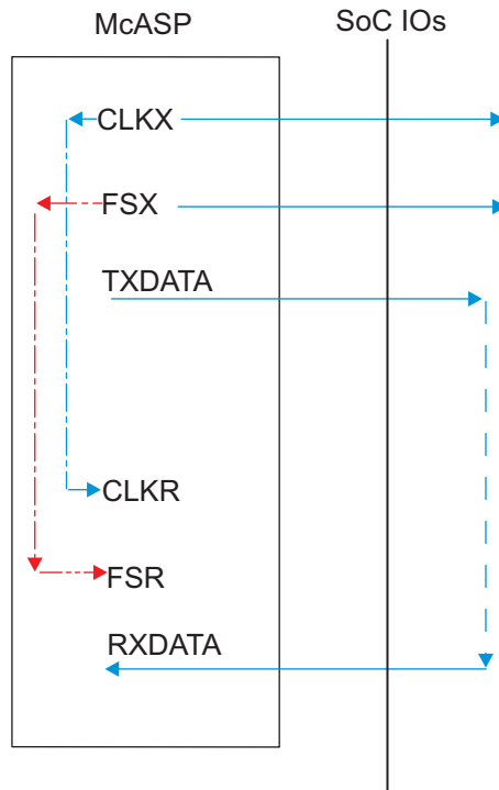
Figure 5-60. McASP1-8 CO-FO- – SYNC Mode
