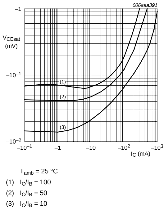
Fig 7. TR1 (PNP): Collector-emitter saturation voltage as a function of collector current; typical values
