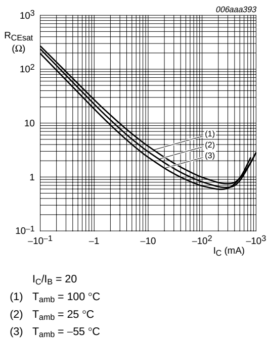
Fig 6. TR1 (PNP): Collector-emitter saturation resistance as a function of collector current; typical values
