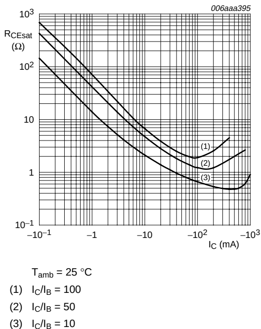
Fig 8. TR1 (PNP): Collector-emitter saturation resistance as a function of collector current; typical values
