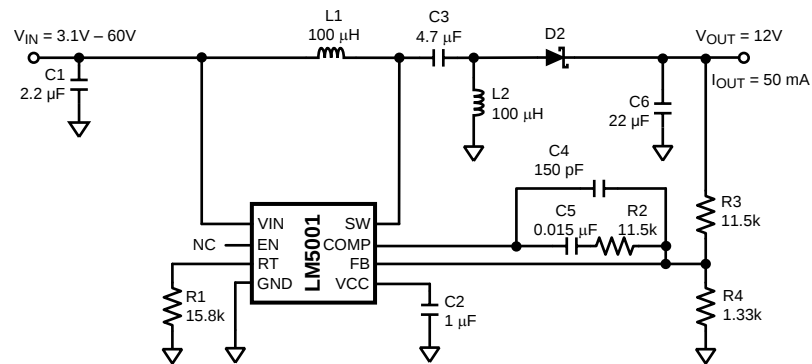
Figure 22. 12-V SEPIC
