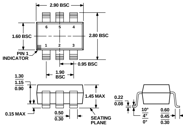
Figure 74. 6-Lead Small Outline Transistor Package [SOT-23] (RT-6)
