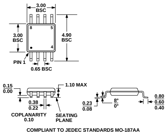
Figure 73. 8-Lead Mini Small Outline Package [MSOP] (RM-8)
