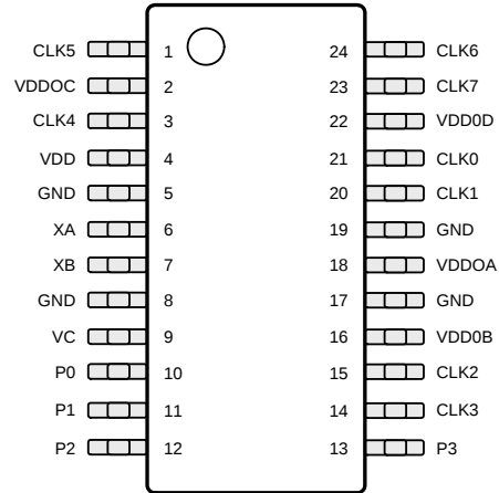
Si5350B 24-QSOP
