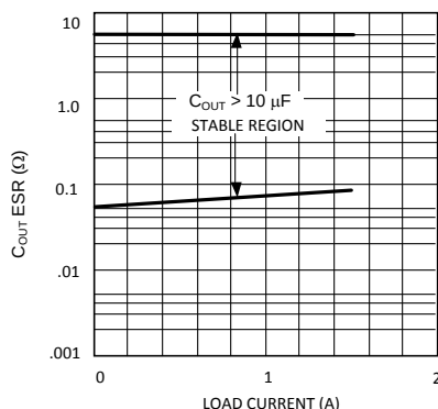
Figure 14. ESR Curve
