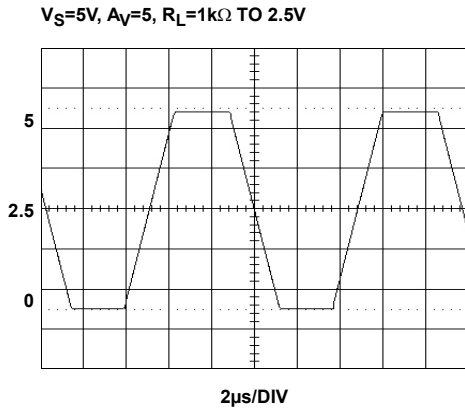
FIGURE 25. OUTPUT SWING
