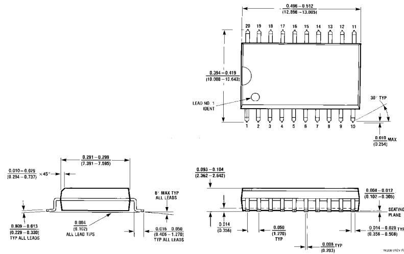
20-Lead Wide Small Outline Molded Package (M) Order Number DM74LS240WM or DM74LS241WM Package Number M20B
