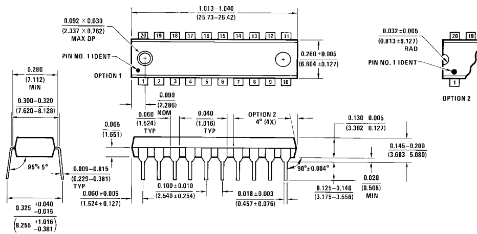
20-Lead Molded Dual-In-Line Package (N) Order Number DM74LS240N or DM74LS241N Package Number N20A
