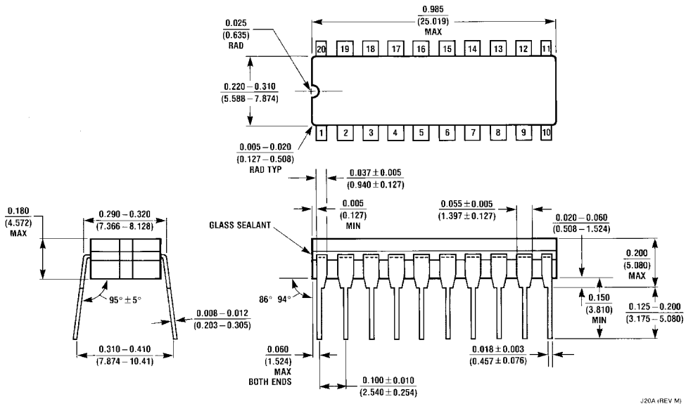
20-Lead Ceramic Dual-In-Line Package (J) Order Number DM54LS240J or DM54LS241J Package Number J20A
