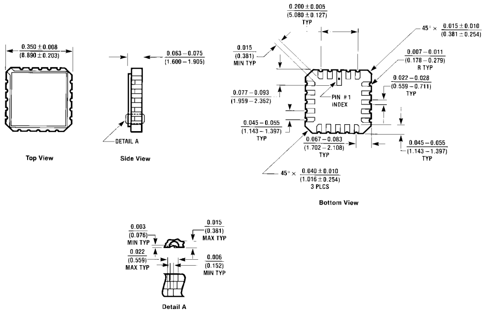
Ceramic Leadless Chip Carrier Package (E) Order Number DM54LS240E or DM54LS241E Package Number E20A
