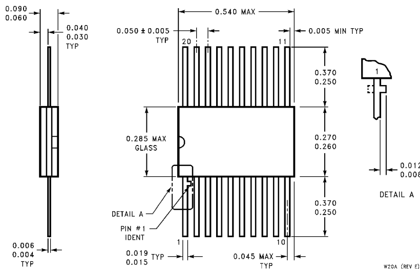
20-Lead Ceramic Flat Package (W) Order Number DM54LS240W or DM54LS241W Package Number W20A
