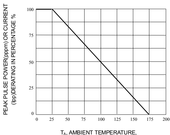
Fig. 2-PULSE DERATING CURVE
