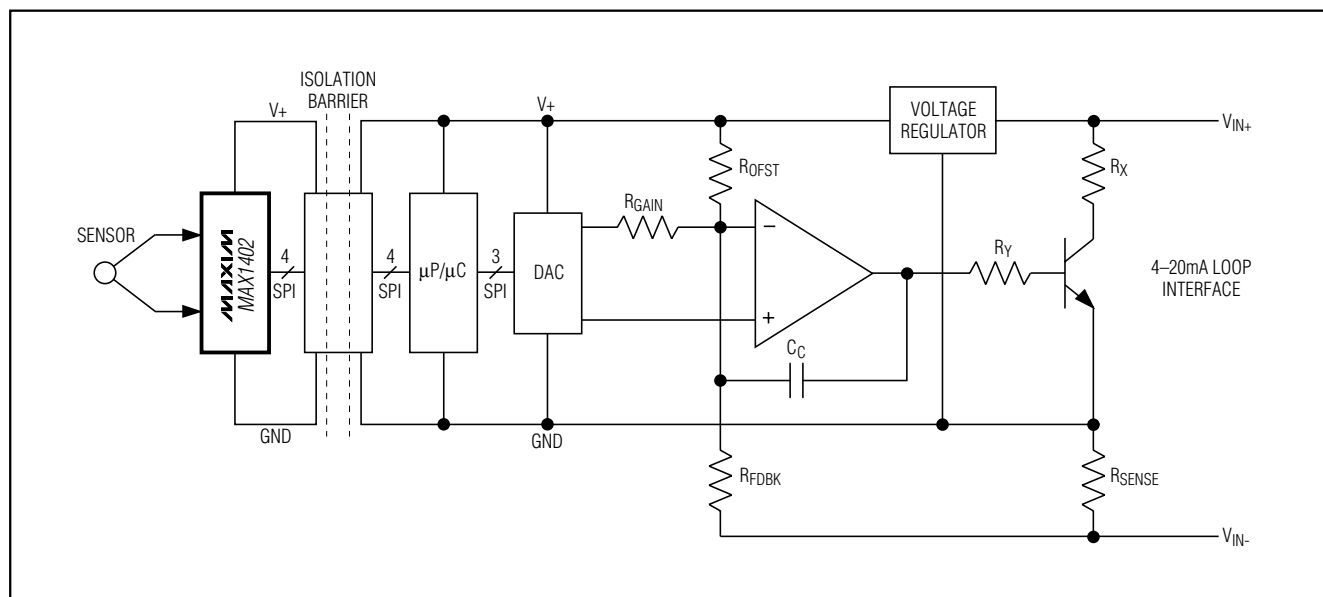
Figure 18. 4–20mA Transmitter
