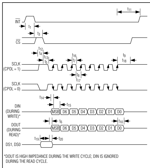
Figure 4. Serial-Interface Timing
