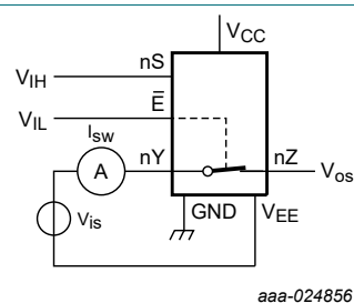
Fig. 10. Test circuit for measuring ON-state leakage current
