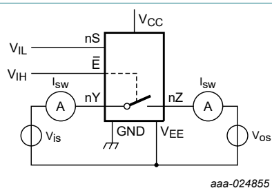
Fig. 9. Test circuit for measuring OFF-state leakage current
