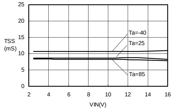
TSS-VIN S-8520/21(Fosc:180kHz)
