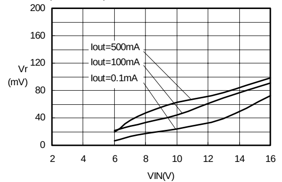
(16) Ripple voltage-VIN S-8521D50MC(Cout:47uFx2)
