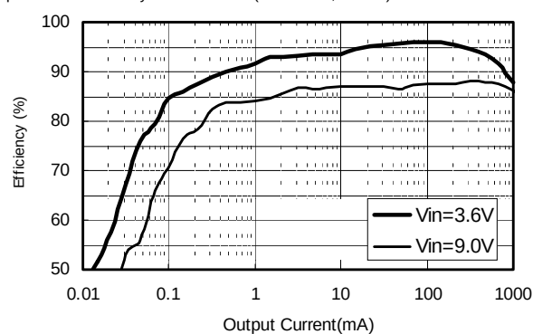
(6) S-8520B50MC Output Current-Efficiency Characteristics (CD54/47uH,TM6201)
