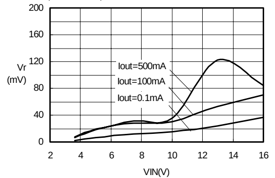
(10) Ripple voltage-VIN S-8521B30MC(Cout:22uFx2)
