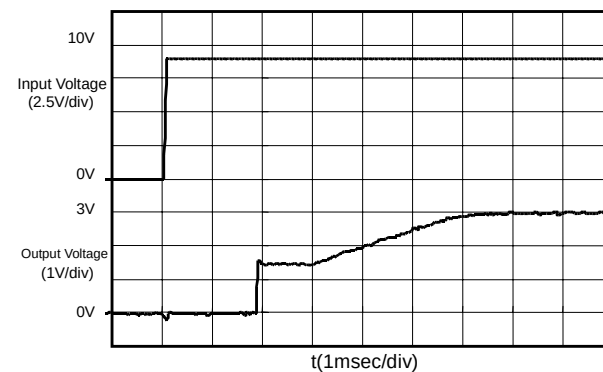
S-8520C30MC ( V_{in}: 0 \rightarrow 9.0V )
