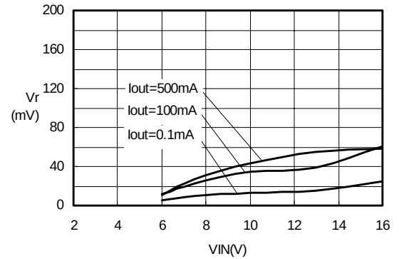
(14) Ripple voltage-VIN S-8521B50MC(Cout:22uFx2)
