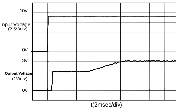
S-8521C30MC ( V_{in}: 0 \rightarrow 9.0V )
