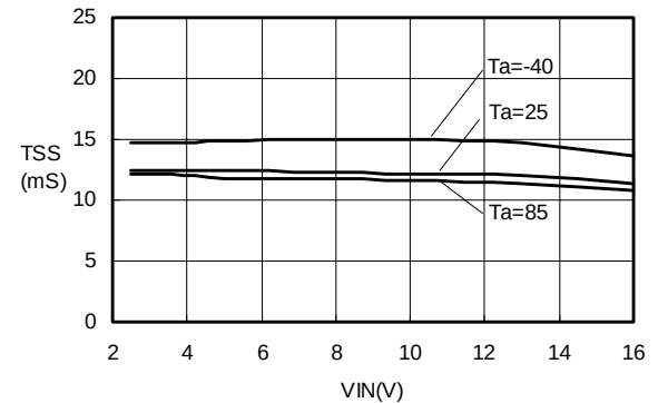
TSS-VIN S-8520/21(Fosc:60kHz)
