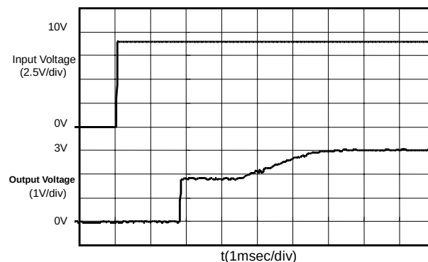
S-8521A30MC ( V_{in}: 0 \rightarrow 9.0V )
