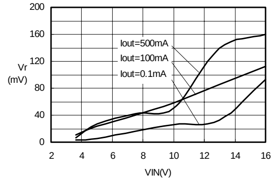
(12) Ripple voltage-VIN S-8521D30MC(Cout:47uFx2)
