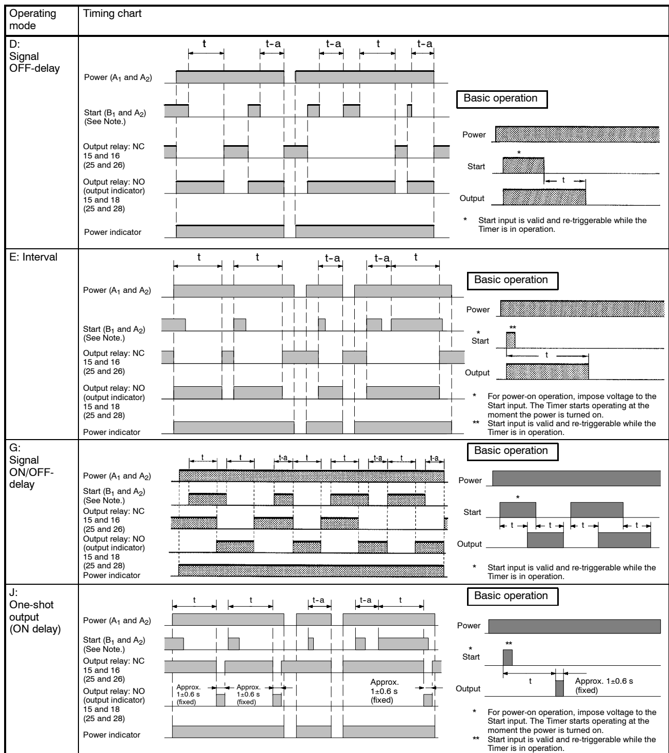
Timing Chart — continued from previous page
