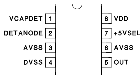
DIL-8, SOIC-8 (Top View) N or D Packages
