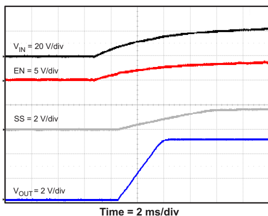
Figure 51. TPS54336 Start Up Relative to VIN
