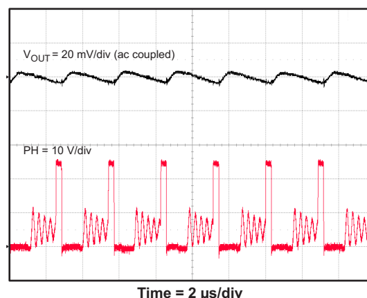
Figure 31. TPS54335 100 mA Output Ripple
