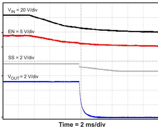
Figure 53. TPS54336 Shut Down Relative to VIN
