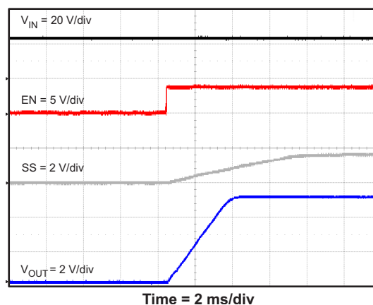
Figure 52. TPS54336 Start-up Relative to Enable
