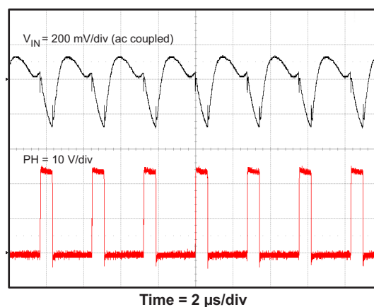
Figure 50. TPS54336 Full Load Input Ripple
