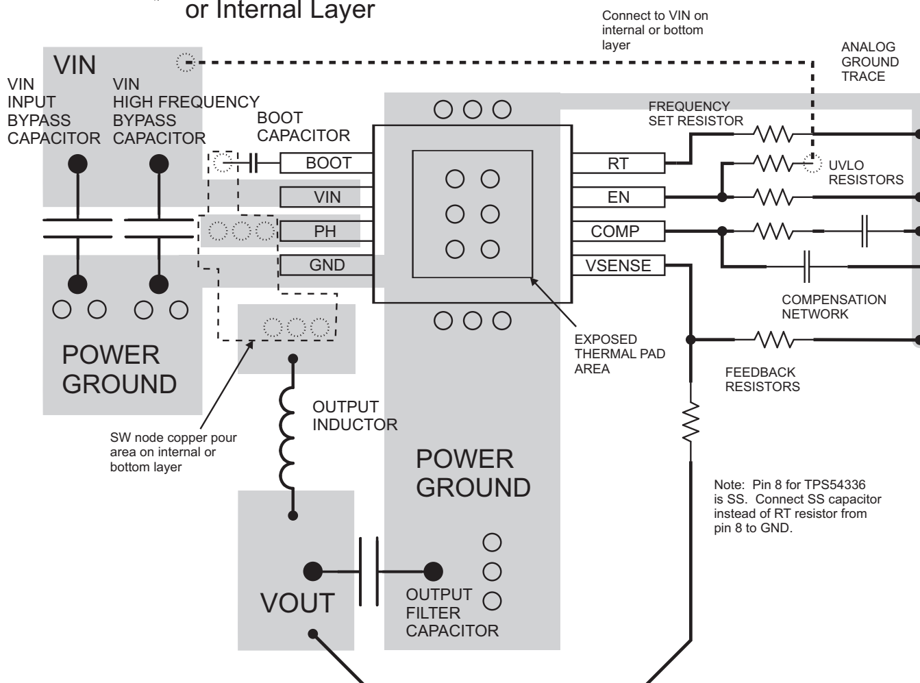
Figure 23. TPS54335DDA Board Layout
