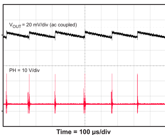
Figure 32. TPS54335 No Load Output Ripple
