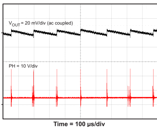
Figure 49. TPS54336 No Load Output Ripple
