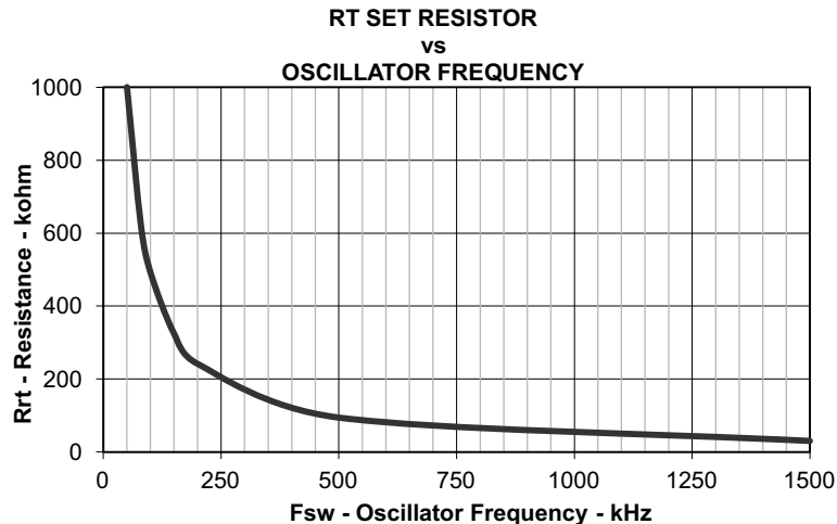
Figure 16. RT Set Resistor vs Switching Frequency
