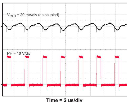
Figure 30. TPS54335 Full Load Output Ripple
