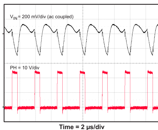
Figure 33. TPS54335 Full Load Input Ripple
