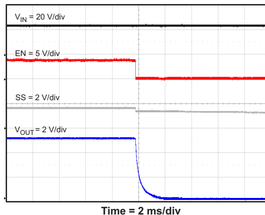
Figure 54. TPS54336 Shut Down Relative to EN
