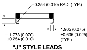
"J" STYLE LEADS
