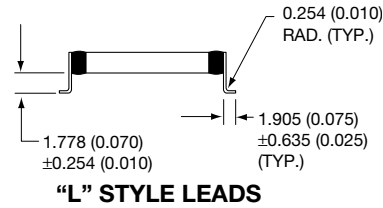
"L" STYLE LEADS
