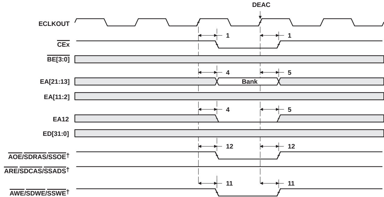
Figure 41. SDRAM DEAC Command
