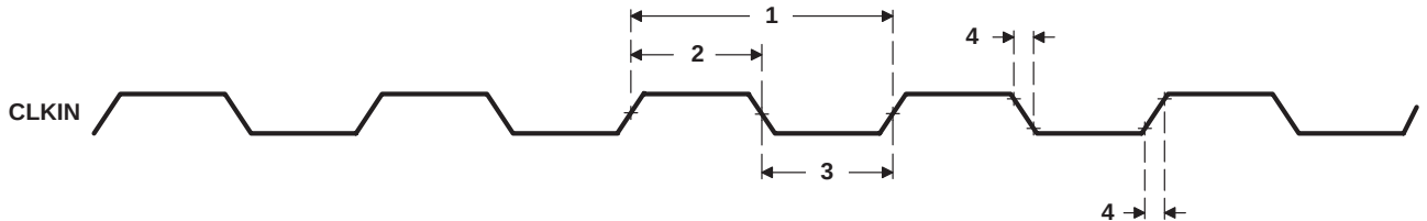
Figure 28. CLKIN Timings
