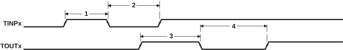
Figure 62. Timer Timing
