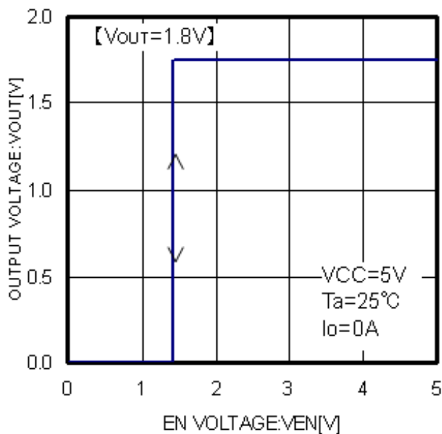
Figure 12. V_{OUT} VS V_{EN}
