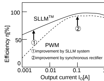
Figure 5. Efficiency
