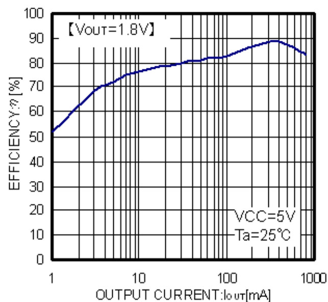
Figure 15. Efficiency
