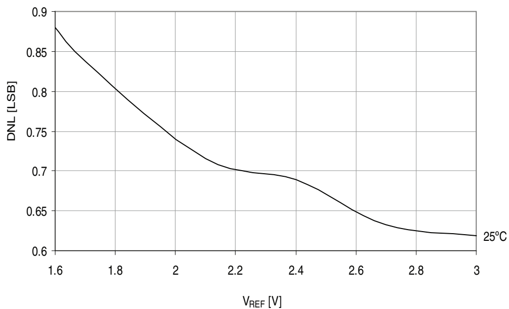
Figure 37-305. DNL error vs. V_{REF} .
