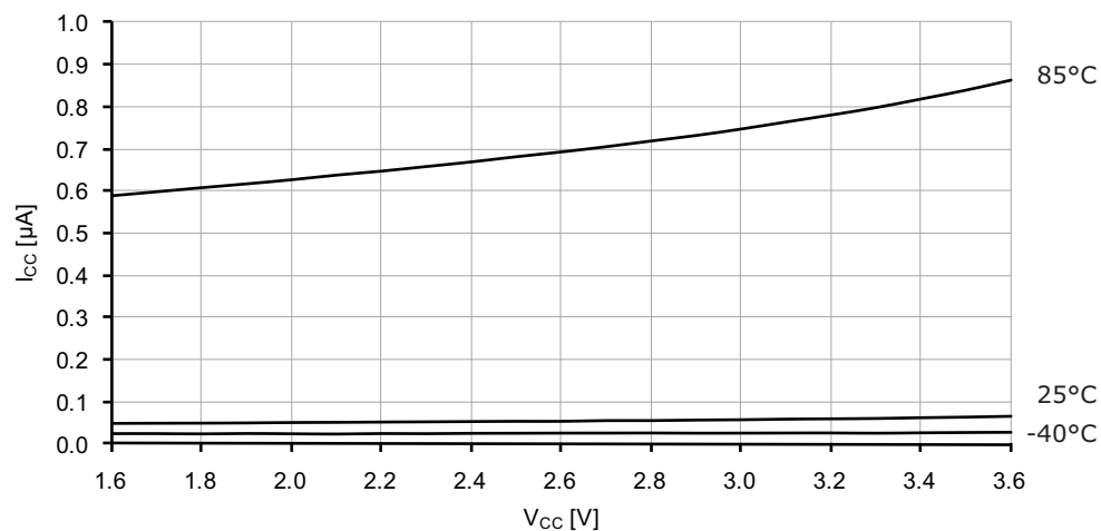
Figure 37-186. Power-down mode supply current vs. V_{CC} .
