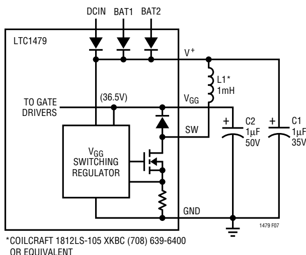
Figure 7. V GG Step-Up Switch Regulator
