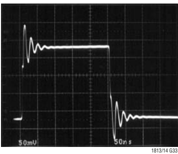
Small-Signal Transient ( A_V = 1 , C_L = 100\text{pF} )
