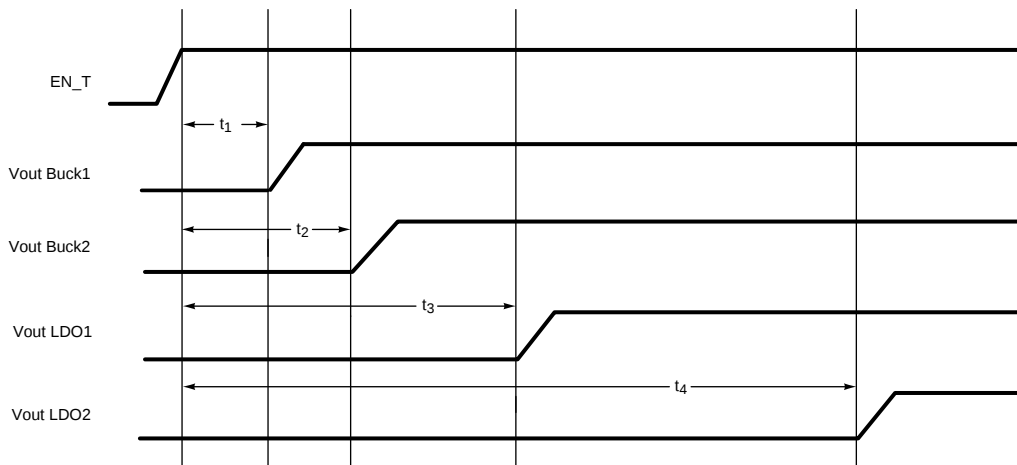
Figure 33. LP3907 Default Power-Up Sequence
