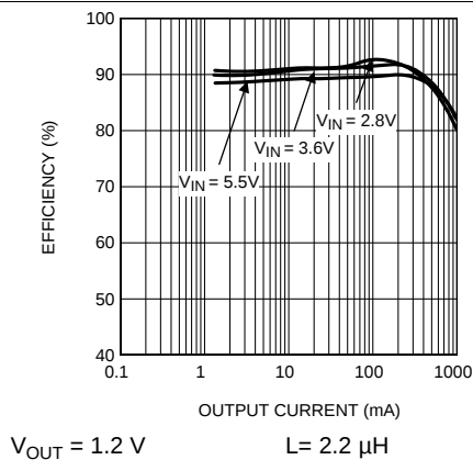
Figure 16. Efficiency vs Output Current (PWM-to-PFM Mode)
