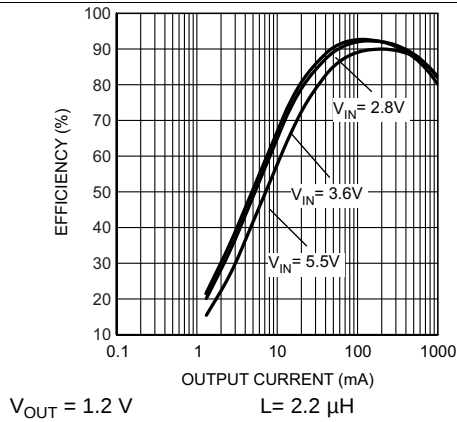
Figure 14. Efficiency vs Output Current (Forced PWM Mode)
