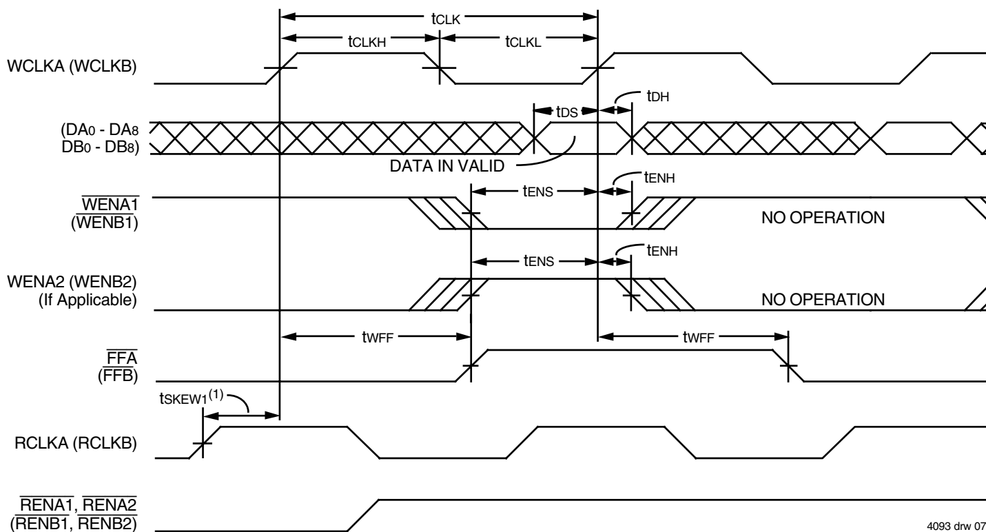
Figure 4. Reset Timing
