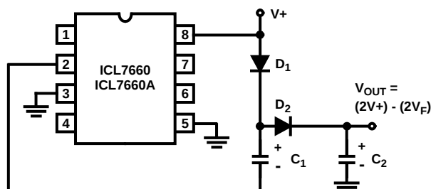
FIGURE 19. POSITIVE VOLTAGE DOUBLER
