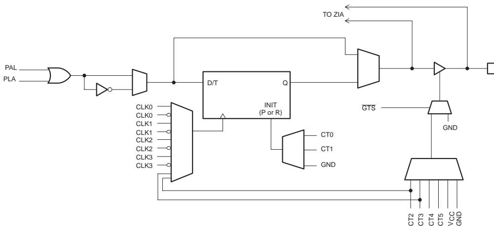
Figure 3: XCR5128C Macrocell Architecture
