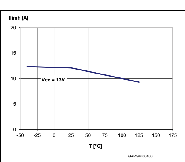
Figure 31. I_{LIMH} vs. T_{case}
