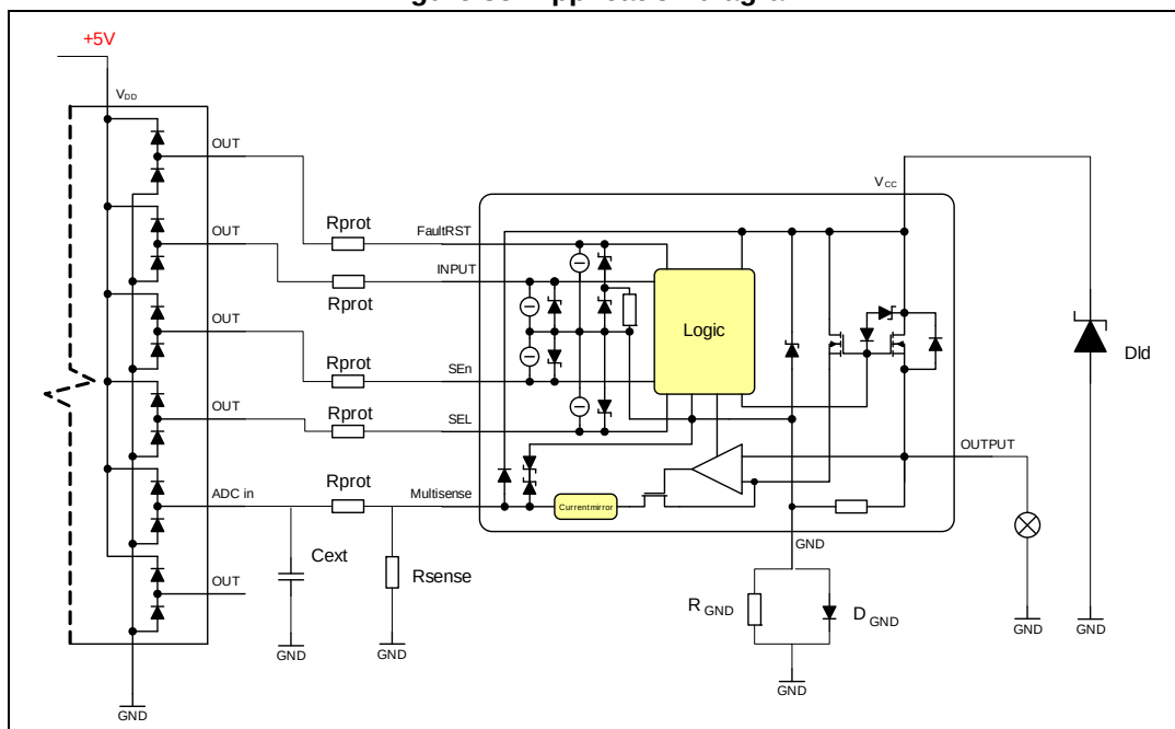
Figure 35. Application diagram
