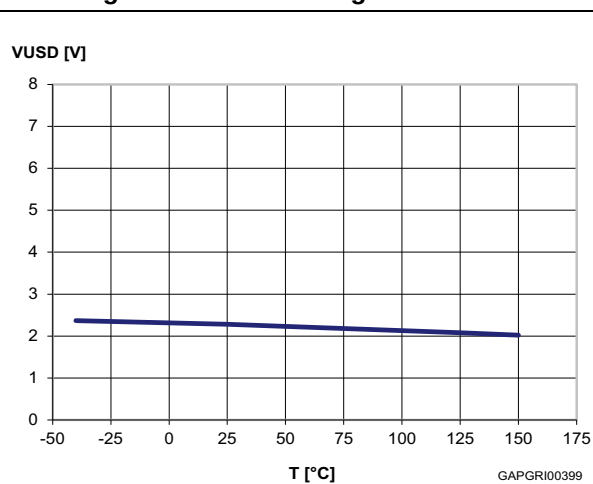
Figure 24. Undervoltage shutdown
