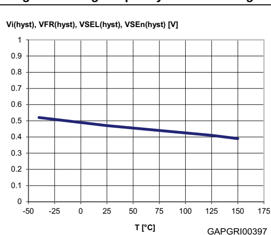
Figure 22. Logic Input hysteresis voltage
