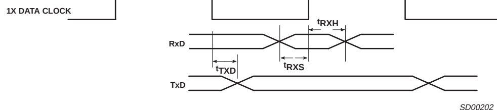
Figure 11. Transmitter and Receiver Timing
