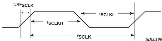
Figure 8. SCLK Timing
