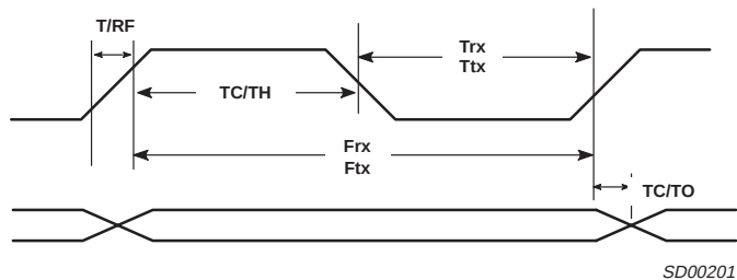
Figure 10. Tx/Rx Clock Timing, External
