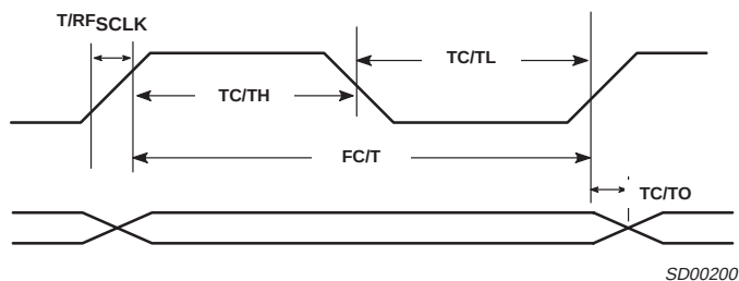
Figure 9. Counter/Timer Baud Rate Clock, External
