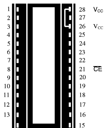
28-Pin Intelligent Socket
