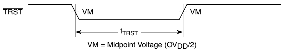
Figure 25. \overline{\text{TRST}} Timing Diagram
