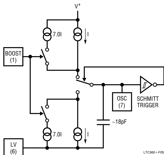
Figure 5. Oscillator
