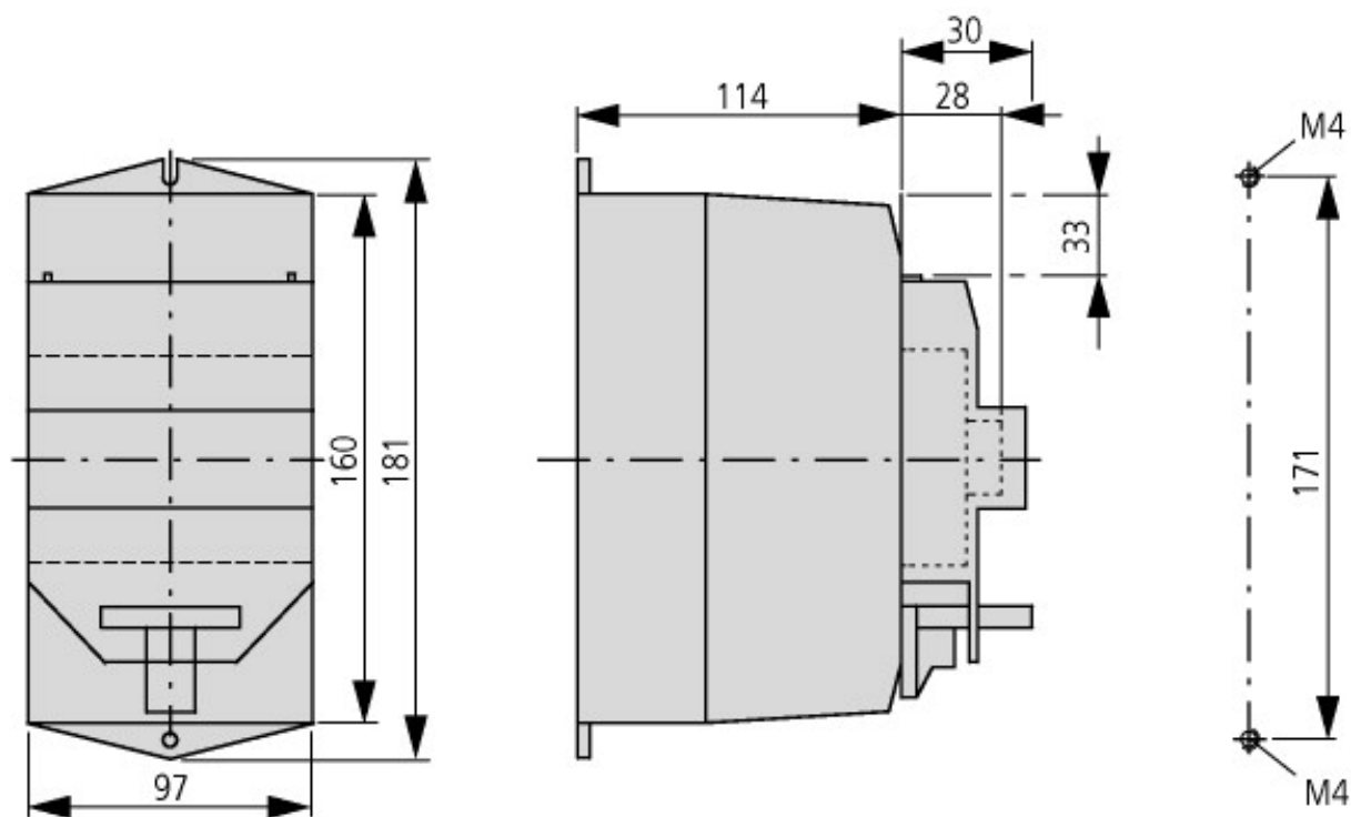
Drilling dimensions
