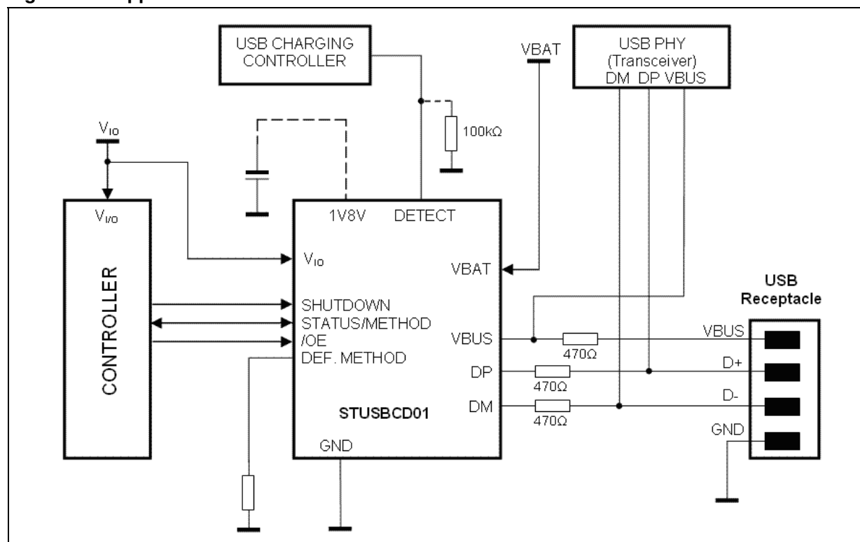
Figure 1. Application circuit
