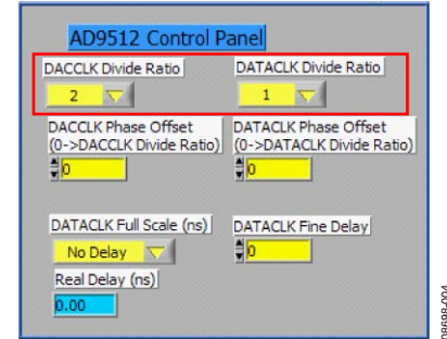
Figure 4. AD9512 Clock Divider Setting
