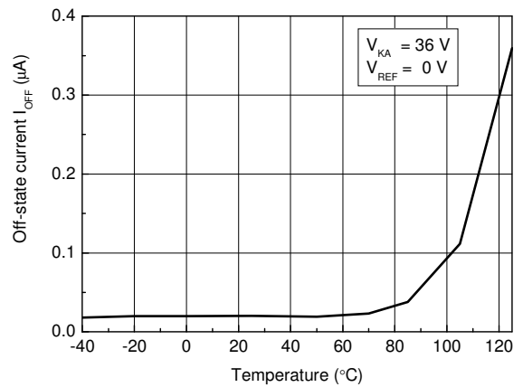
Figure 16. Off-state cathode current vs. temperature
