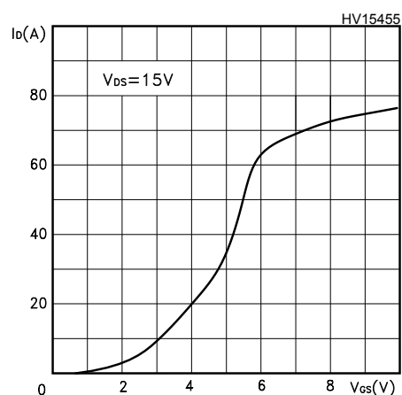
Figure 4. Transfer characteristics
