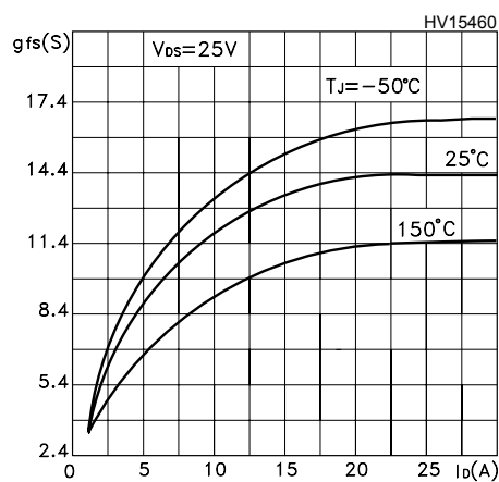
Figure 5. Transconductance
