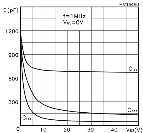
Figure 8. Capacitance variations
