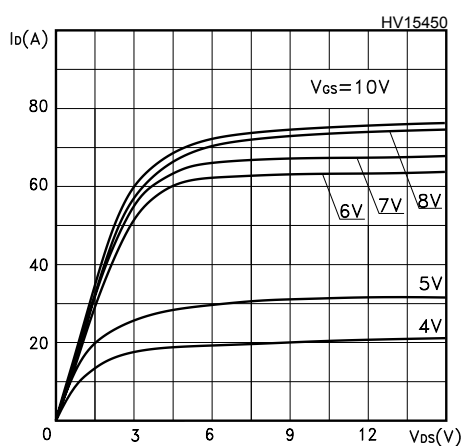
Figure 3. Output characteristics
