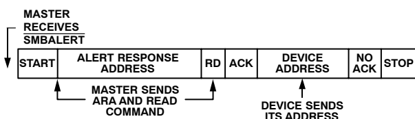
Figure 13. Use of \text{SMBALERT}
