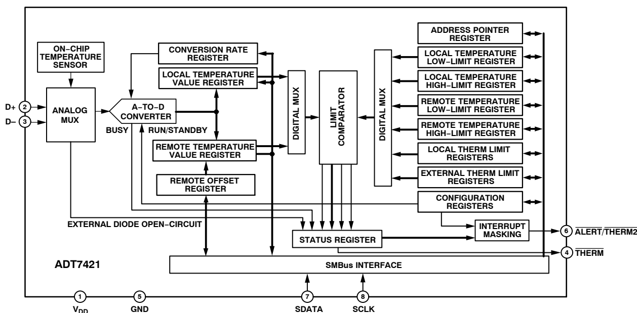
Figure 1. Block Diagram
