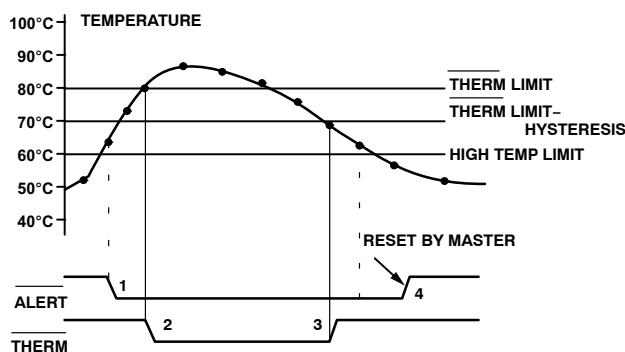
Figure 14. Operation of the \overline{\text{ALERT}} and \overline{\text{THERM}} Interrupts
