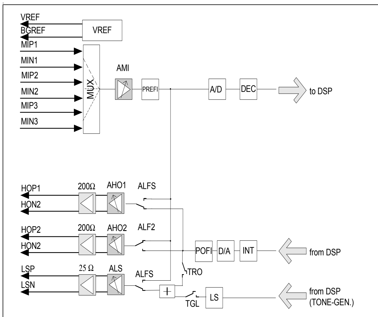
Figure 19-1 Analog Front End
