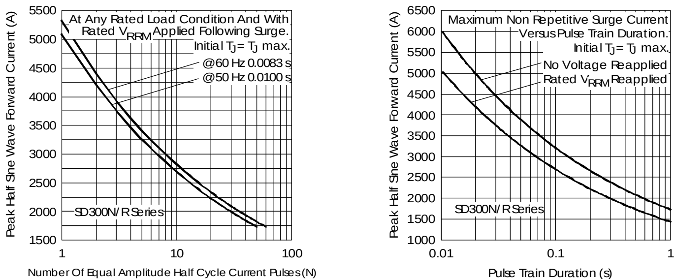
Fig. 9 - Maximum Non-Repetitive Surge Current
