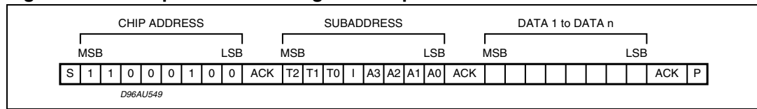
Figure 12. Example for addressing the tuner part:
