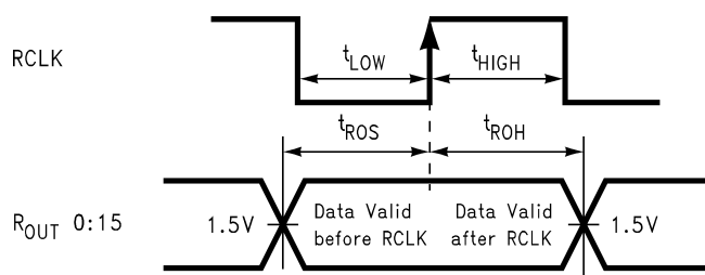
Figure 12. Deserializer Setup and Hold Times
